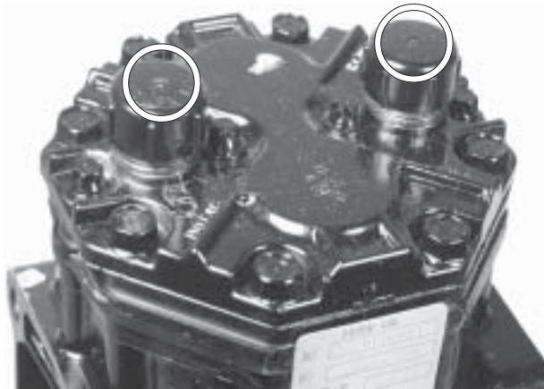
Oil leaking from center of shipping cap. Factory nitrogen charge may cause slight oil leak from center of cap while in box. Check oil level prior to installing compressor.
