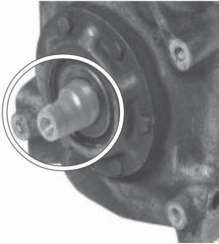
Keyway not properly installed on compressor shaft.
