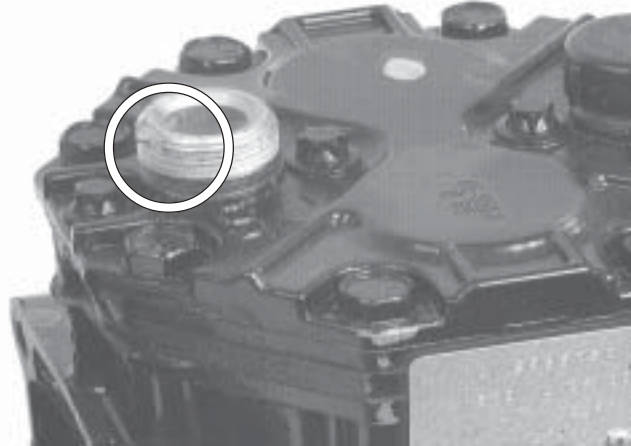
Dropped Compressor shown by the flat dent in threads.
