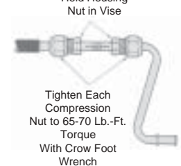
ORIFICE TUBE KIT INSTALLED
