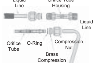
ORIFICE TUBE LOCATION - DISASSEMBLED
